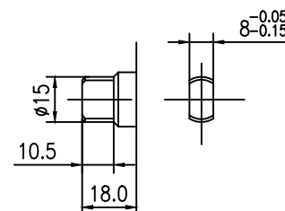
扁键
